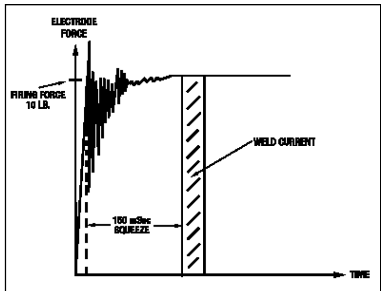
Figure 2: Electrode Force vs. Time for an improperly adjusted weld head
