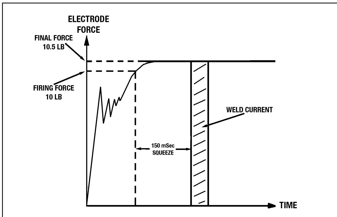
Figure 1: Electrode Force vs. Time for Model 80A Weld Head
