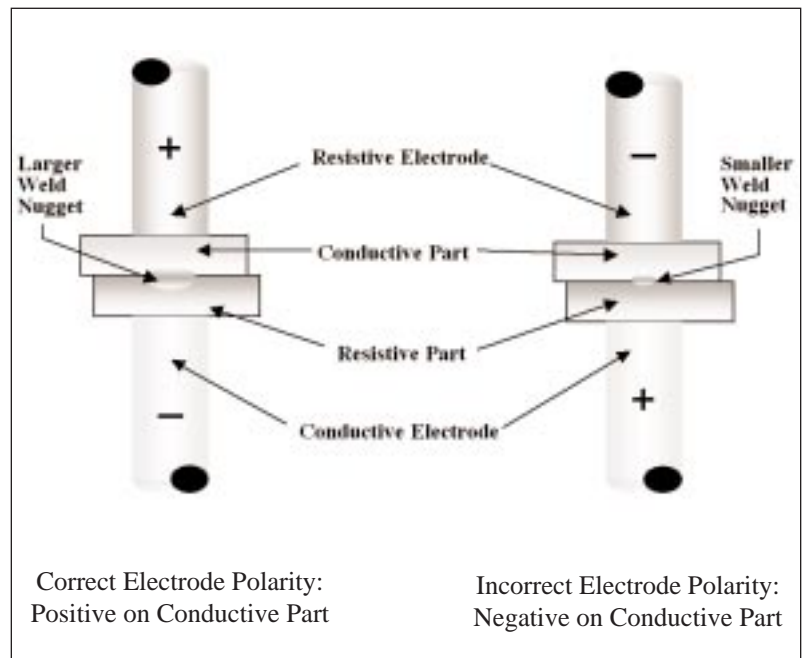
Figure 1: Opposed Weld Polarity Effect
