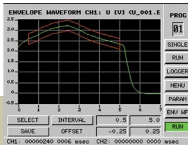
Acceptable – Weld Envelope
